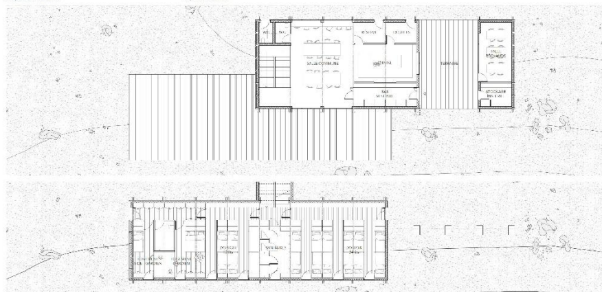
Plans - 1:100
